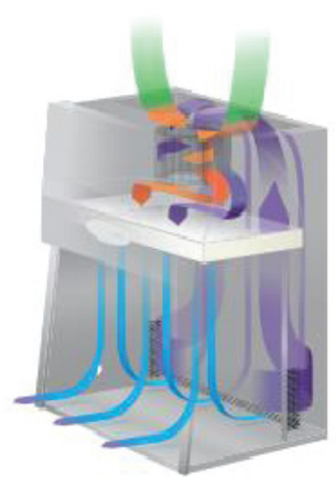
Vertical Laminar Airflow
