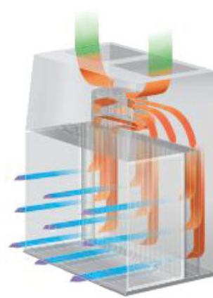
Horizontal Laminar Airflow
